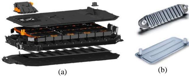
Figure 1. Evaluated use case: (a) battery pack [9]; (b) FLEXcooler [10].
