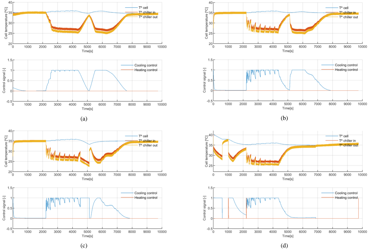
Figure 6. Results from (a) the first simulation, (b) the second simulation, (c) the third simulation and (d) the fourth simulation. There are two figures: the upper figure is the thermal response of the battery and the coolant; the lower figure is the response of the controller.
