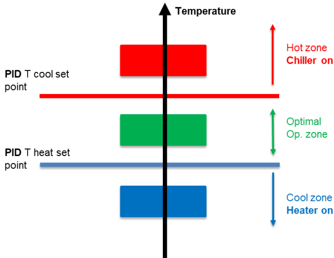
Figure 3. Design of the adaptive and smart control strategy.
