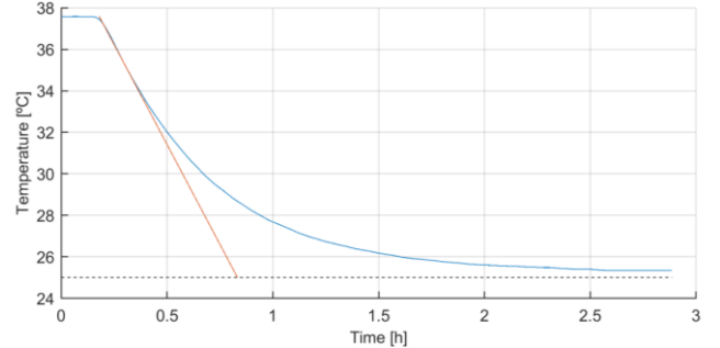
Figure 2. Applied Ziegler-Nichols method for the heat exchanger PID.
